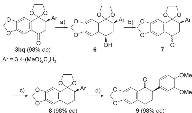
Scheme 3. Transformation of 3bq to 2-aryltetralone 9 . a) LiAlH 4 , THF, 0 °C, 1 h, 94%; b) n -BuLi, THF, 0 °C, 0.5 h; then TsCl, 0 °C to room temperature, 12 h; c) NaBHET 3 , toluene, 0 °C to room temperature, 2.5 h, 61% (2 steps), 98% ee ; d) 10% aqueous HCl, MeOH, −15 °C, 1 h, 81%, 98% ee .
