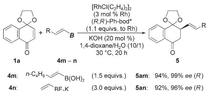
Scheme 1. Asymmetric 1,4-addition of alkenylborons 4 to monoketal 1a catalyzed by Rh/( R,R )-Ph-bod*.
