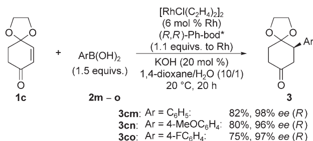
Scheme 2. Asymmetric 1,4-addition of arylboronic acids 2 to dihydrobenzoquinone monoketal 1c .
