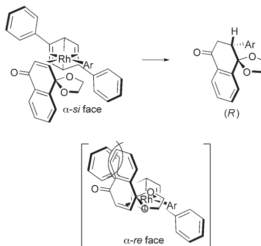
Figure 1. Enantioselection in the rhodium-catalyzed asymmetric 1,4-addition.
